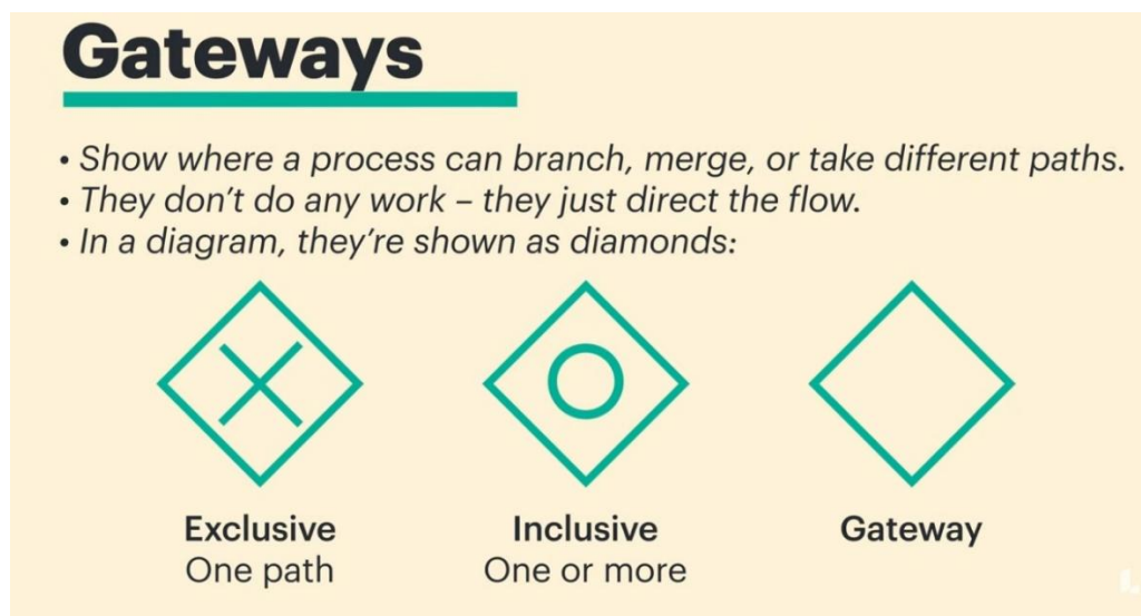
Figure 2 BPMN GATEWAYS
