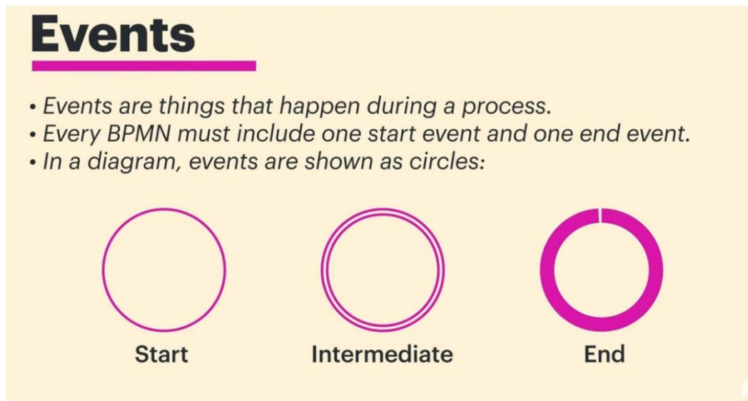
Figure 1 BPMN EVENTS
